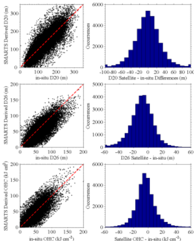
Figure 2-8 - Scatterplots (left) of D20 (top), D26 (middle), and OHC (bottom) comparing In-situ measurements to values derived by the two-layer model using the SMARTS Climatology. Data points with differences greater than 4 standard deviations from the mean were removed (<0.5% of points). Histograms (right) of errors have bin widths of 10 m, 5 m, and 5 \text{kJ cm}^{-2} for D20, D26, and OHC, respectively.
