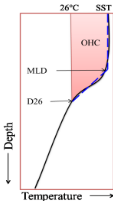
Figure 1-1 - Schematic of OHC calculation. The red shading shows the true OHC by integrating the black temperature profile. The dashed blue line shows the approximated temperature profile of the upper ocean.
