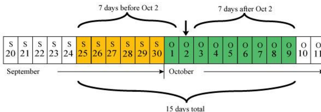
Figure 2-5 - A 15-day running mean was used to create the 'daily' climatology. For example, to create the October 2nd climatology, the September climatology was weighted 6/15 and the October climatology is weighted 9/15.
