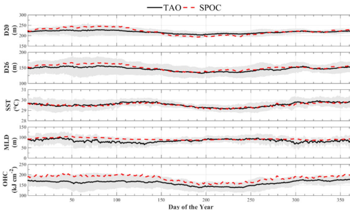
Figure 2-23 - A 17-year averaged time series comparisons of D20, D26, MLD, SST, and OHC from the TAO/TRITON mooring at 8oS, 180o in the central Pacific Ocean. Uncertainty (gray shaded) represents error bars equivalent to 1\sigma over the 17-year period of concurrent In-situ and satellite measurements.
