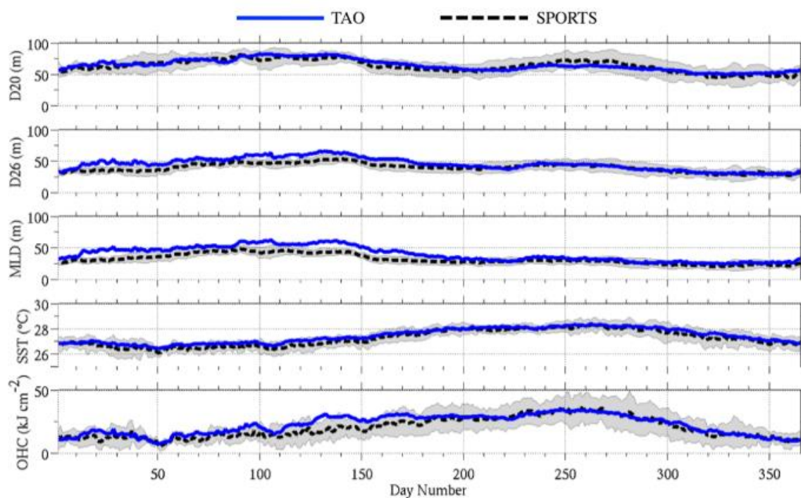
Figure 2-21 - A 12-yr averaged time series comparisons of D20, D26, MLD, SST, and OHC from TAO/TRITON mooring at 90N, 1400W in the central Pacific Ocean where the uncertainty (gray shaded) is represented by error bars equivalent to 1\sigma over the 12-year period of concurrent In-situ and satellite measurements.
