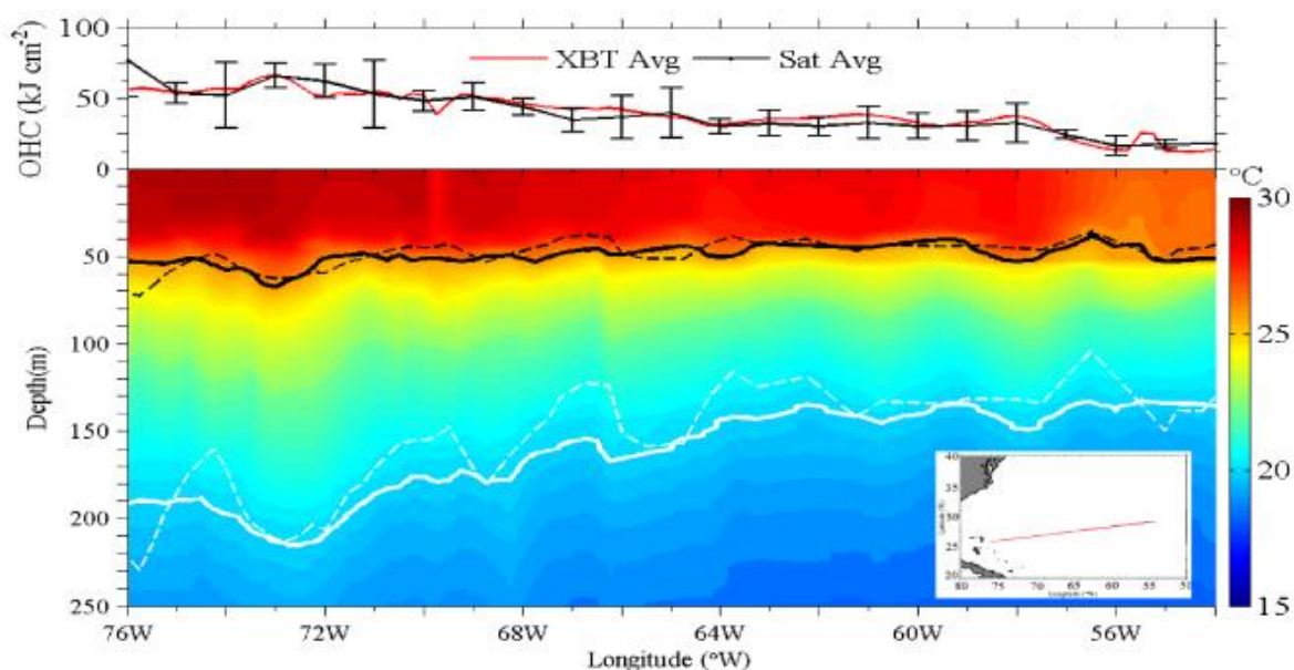
Figure 2-20 - Average temperature observed by XBTs along an east-west transect from 25oN to 28oN (inset) with observed (solid) and SMARTS-derived (dashed) depths of D26 (black) and D20 (white). Observed OHC (red line, top) is compared to satellite derived values with error bars equivalent to 2\sigma .
