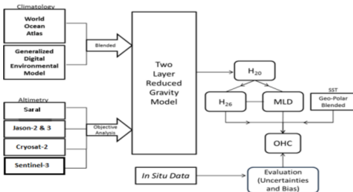
Figure 2-1 - Flow diagram of the inputs to the reduced gravity model including the objectively analyzed SSHA from various radar altimeters to estimate the depth of the 20oC isotherm which is then used to determine the depth of the 26oC isotherm and MLD and the GEO-POLAR SST to calculate OHC. In situ data includes temperature profiles from Argo floats, XBT transects, AXBTs deployed from research aircraft, PIRATA moorings in the North Atlantic Ocean Basin and TAO/TRITON moorings in the Pacific Ocean Basin.
