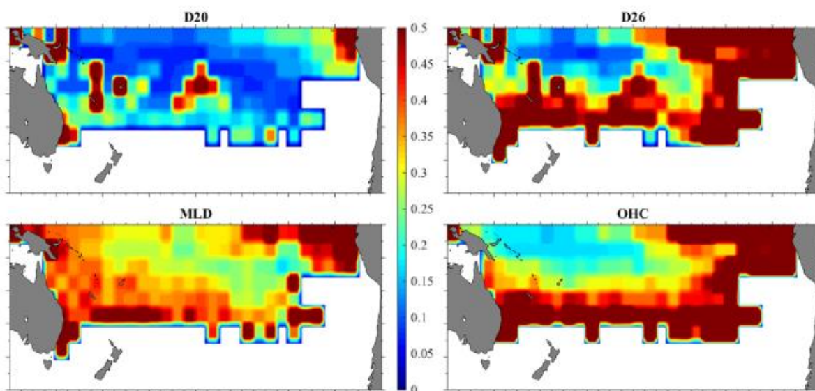
Figure 2-18 - Normalized RMSD for D20, D26, MLD, and OHC during the Cyclone season. The contours represent the differences relative to the variables' average magnitudes for the South Pacific Ocean Basin.
