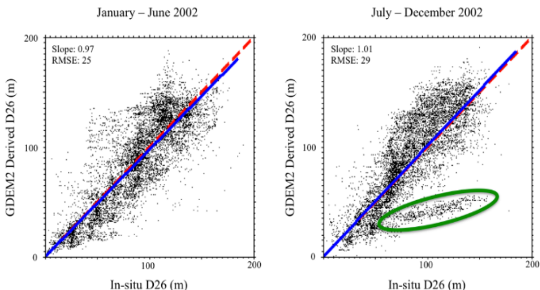
Figure 2-15 - Regression analysis of In-situ versus GDEM2 climatology derived D26 for the North Pacific Ocean basin for 2002 with January through June on the left and July through December on the right. The red dashed line represents the 1:1 ratio line, the blue line represents the best-fit line, and the green circle highlights the anomalous signal.
