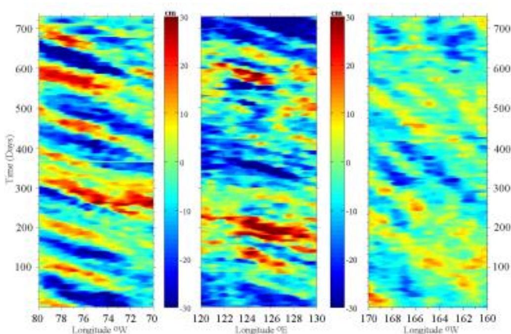
Figure 2-6 - Hovmöller of SSHA at 15°N in Caribbean Sea (left), at 25°N in the Western North Pacific Ocean Basins (middle), and at 25°S in the South Pacific for two years. Drift velocities are on the order of 0.1°/day compared to previous estimates of as much as 0.3°/day.
