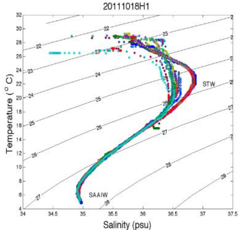
Figure 3-1 - Temperature and salinity diagrams for AXCTDs deployed during a LC survey over the GOA in October 2011 from NOAA WP-3D. Solid contours are sigma-t. The water masses are marked accordingly where the STW (subtropical water) emanates from the Caribbean Sea and is the classic signature of the LC and WCR and SAAIW is Sub Antarctic Intermediate Water.
