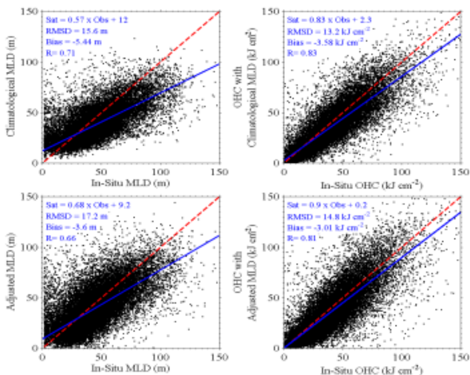
Figure 2-9 - Scatterplots of MLD (left) and OHC (right) comparing In-situ observations to satellite estimations using climatological MLD (top) and the adjusted MLD (bottom). The red dashed line represents a 1:1 relationship and the linear regression line is solid blue.
