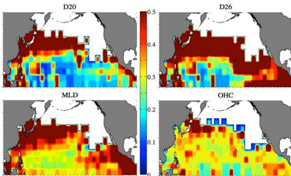
Figure 2-17 - Normalized RMSD for D20, D26, MLD, and OHC during the hurricane season. The contours represent the differences relative to the variables' average magnitudes for the North Pacific Ocean Basin.
