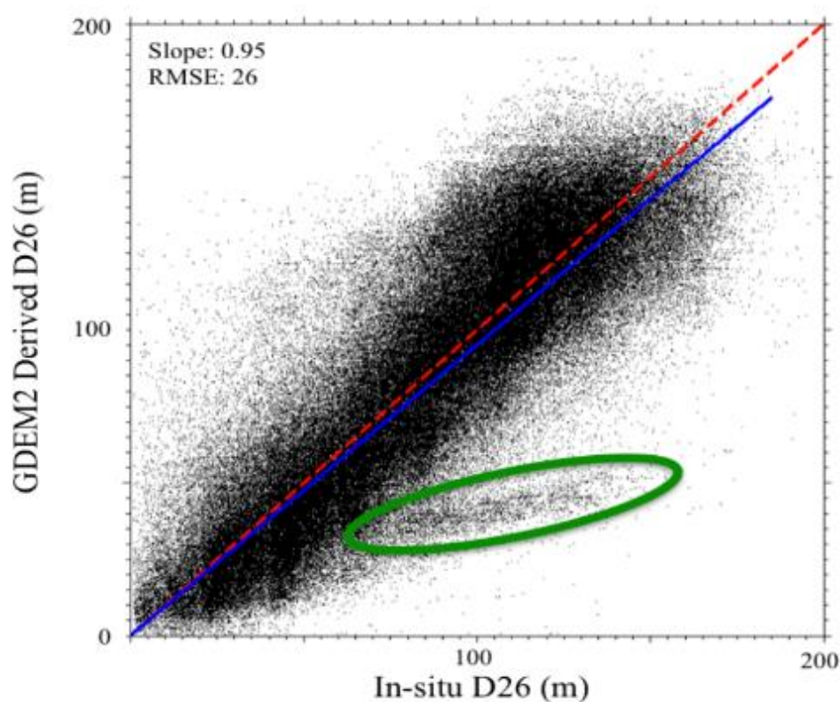
Figure 2-14 - Regression analysis of In-situ versus GDEM2 climatology derived D26 for the North Pacific Ocean basin from 2000-2011. The red dashed line represents the 1:1 ratio line, the blue line represents the best-fit line, and the green circle highlights the anomalous signal.
