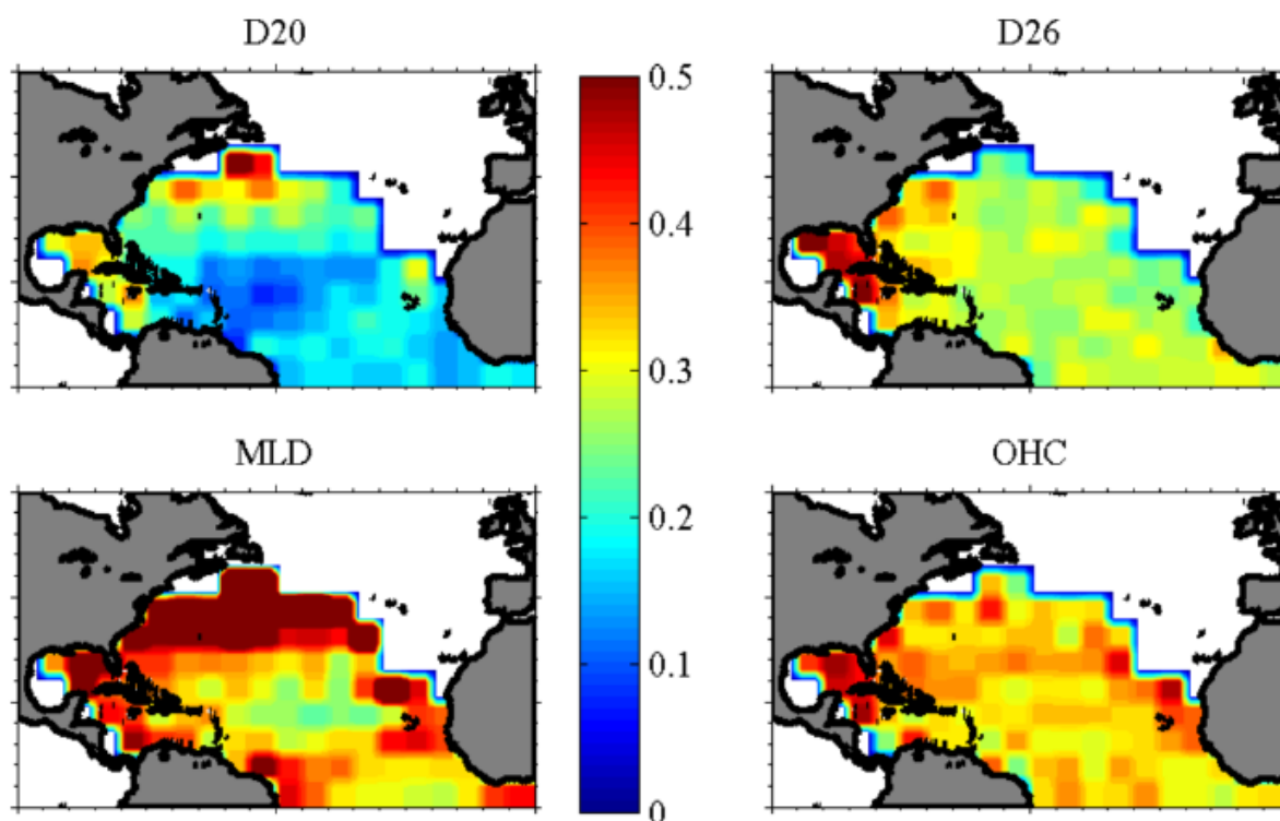
Figure 2-16 - Normalized RMSD for D20, D26, MLD, and OHC during the hurricane season. The contours represent the differences relative to the variables' average magnitudes. NRMSD is greatest in the GOA and northern Atlantic.
